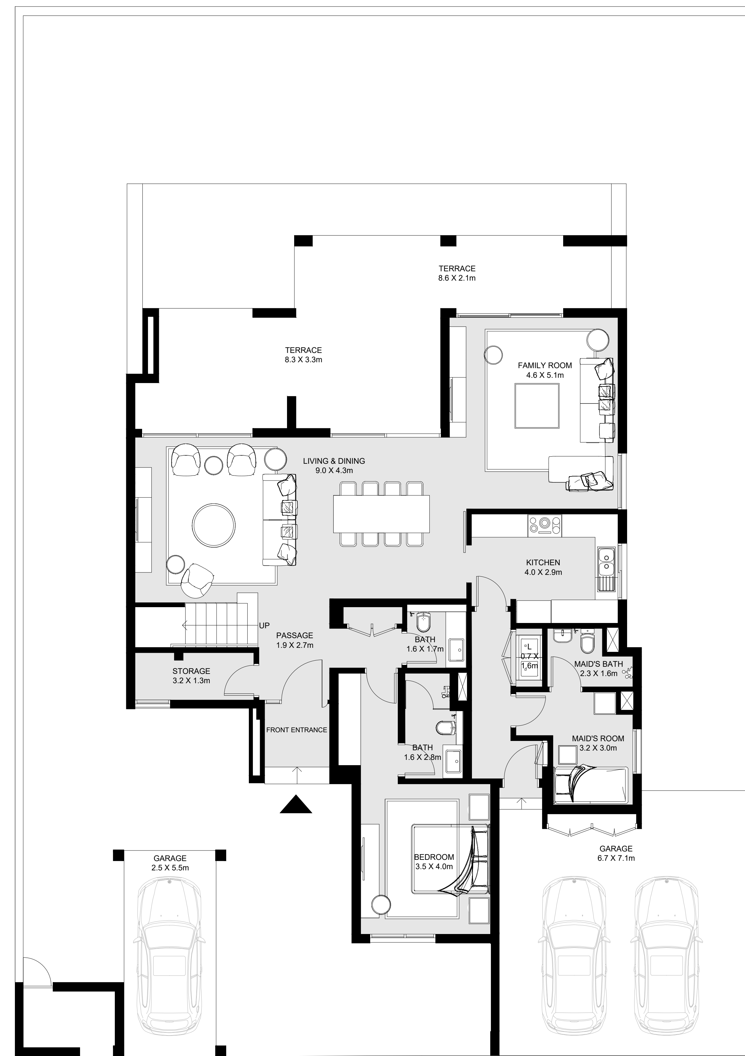
GROUND FLOOR
