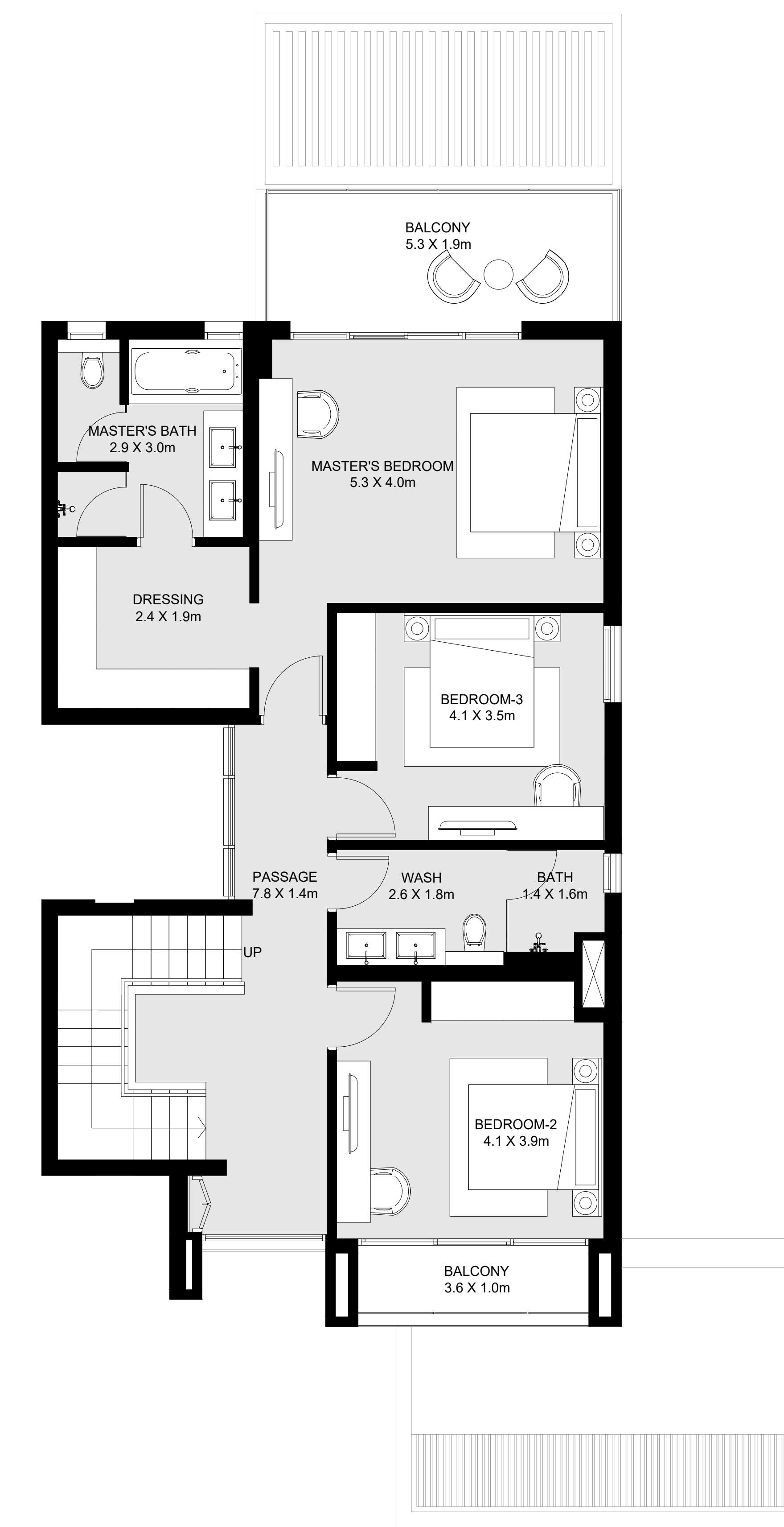
FIRST FLOOR
