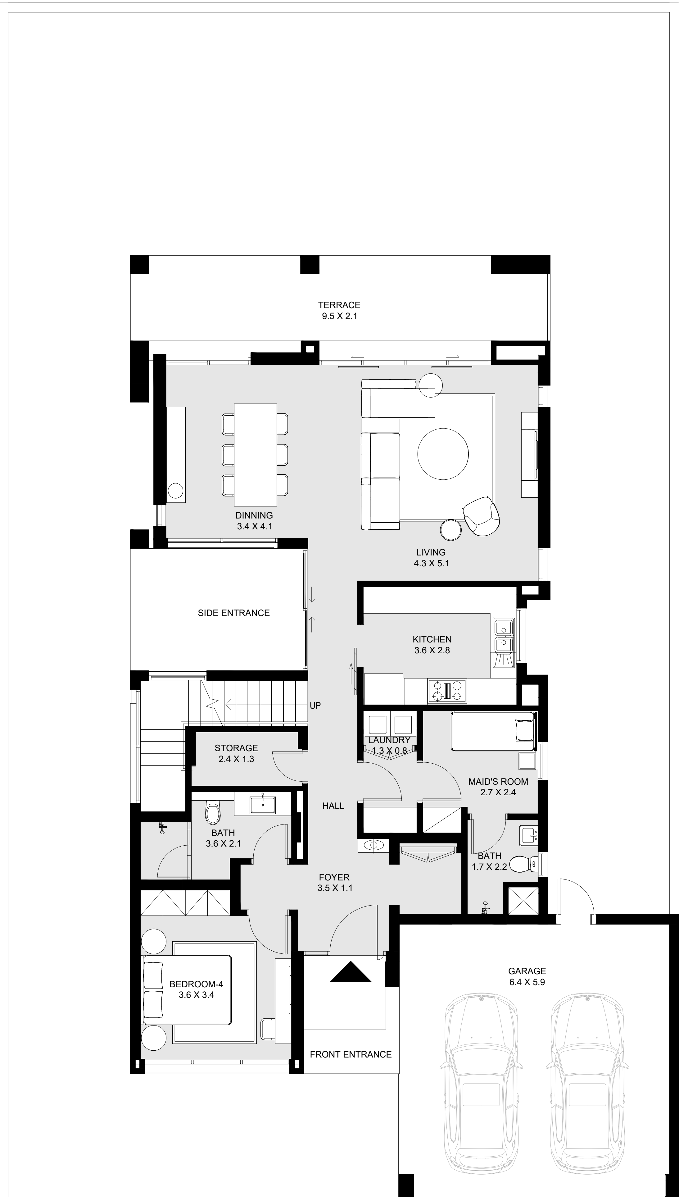
GROUND FLOOR
